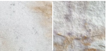
Homokkő / Sandstone
