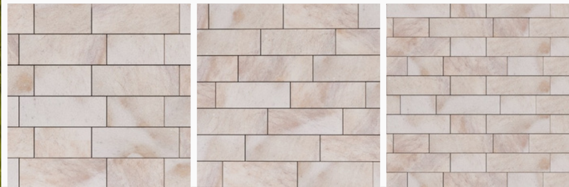
Homokkő / Sandstone
