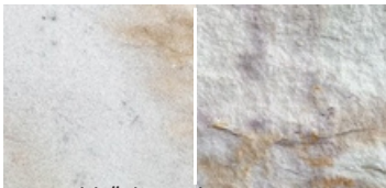
Homokkő / Sandstone
