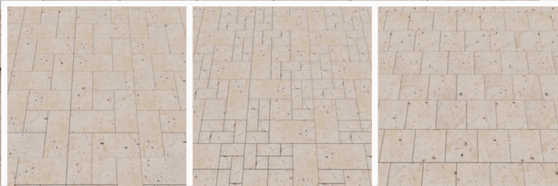
Homokkő / Sandstone
